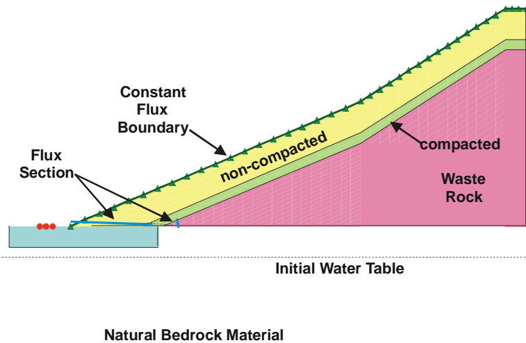
Figure 4.7 Example of a “barrier” layer cover system on a sloping waste rock surface.
