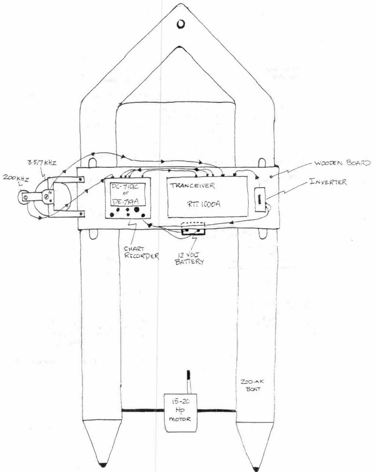
Fig.1 Rathyeon 1000 subbottom acoustic profiler set up
