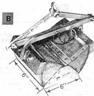
PETITE PONAR GRAB SAMPLER Catalog No. 1728
