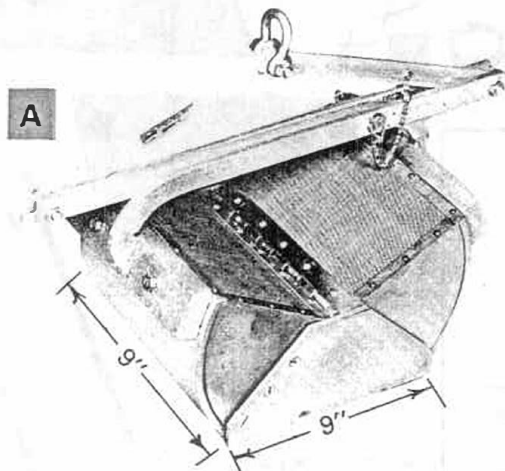
PONAR GRAB SAMPLER Catalog No. 1725
