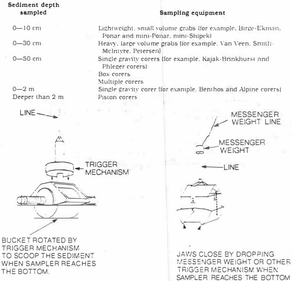
FIGURE 2. Grab samplers with their essential parts. (Mudrock and Hackright, 1991)
