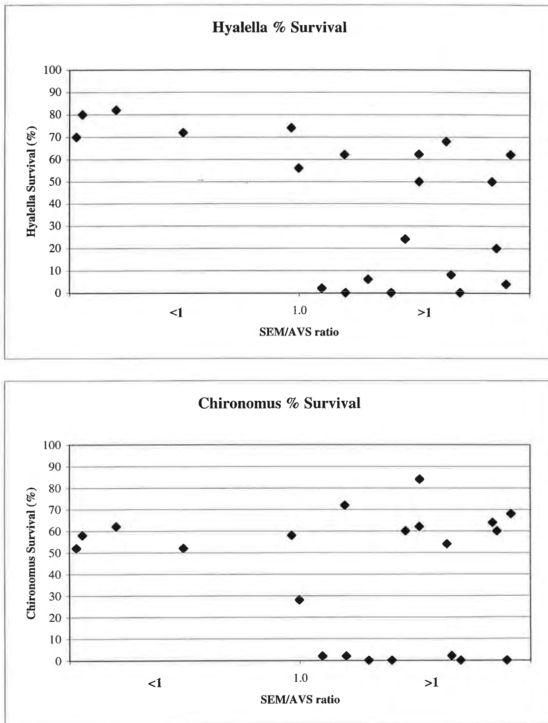
Figure 5.6: Sediment Toxicity versus Ratio of Simulatneously Extracted Metals (Cd+Cu+Ni+Pb+Zn)/Acid Volatile Sulphide. Myra Falls, September 1997.
