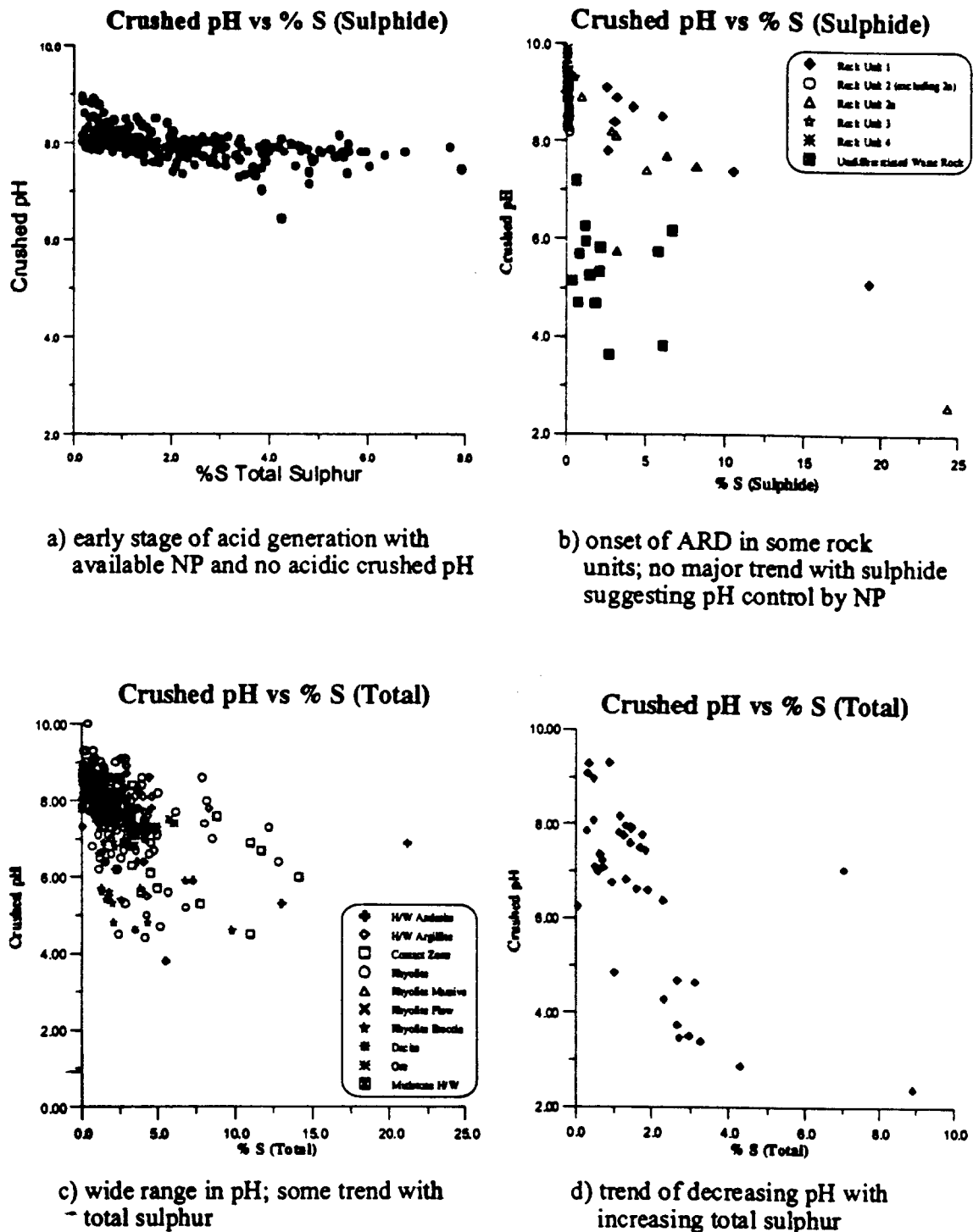
Figure 8-3 Scatterplots of Total/Sulphide Sulphur vs. Crushed pH from B.C. Mines
