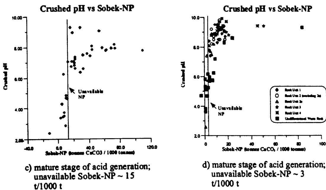
Figure 8-4 Scatterplots of Sobek-NP vs. Crushed pH from B.C. Mines
