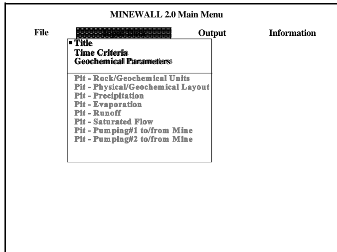
FIGURE 3-7. The Input Data Submenu after the Title Form has been completed.
