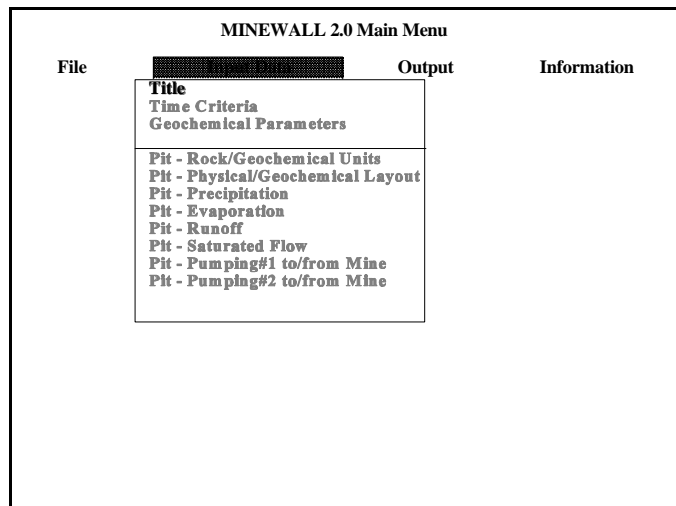
FIGURE 3-5. The Input Data Submenu with the Title selection enabled.
