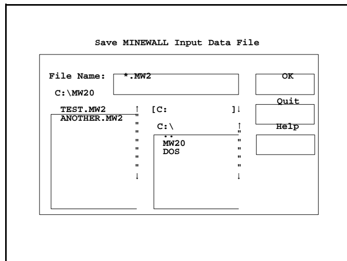
FIGURE 5-3. The Save Current Data Form.
